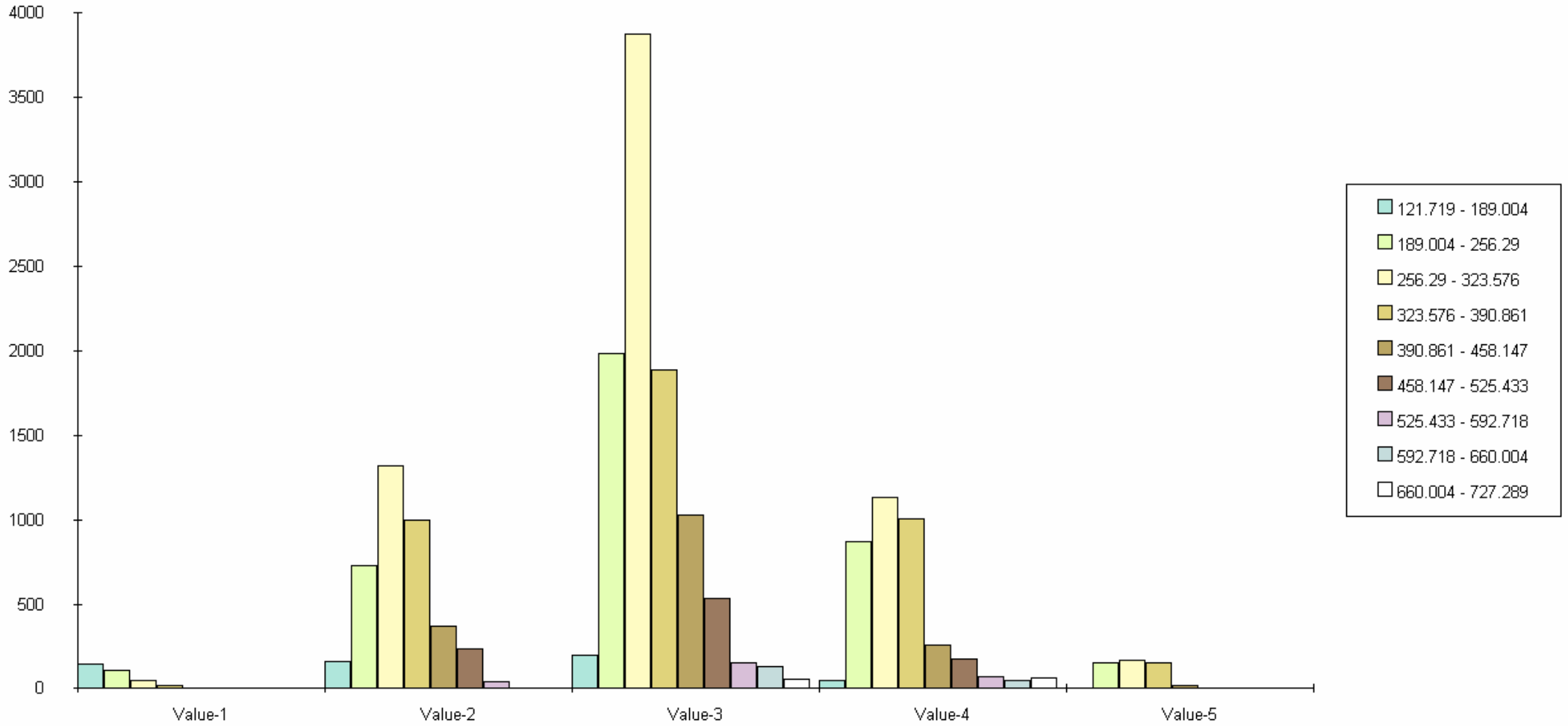
Histogram of Potassium Content:Value
